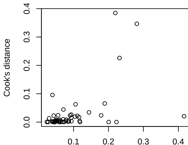
Cook's dist vs Leverage
